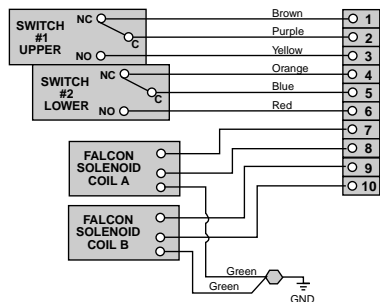
2-SPDT Mechanical Switches with Falcon Dual Coil Solenoid & 10 PT TS
