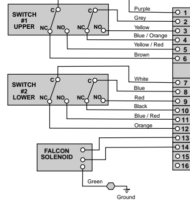
2-DPDT Mechanical Switches with Falcon Dual Coil Solenoid & 16 PT TS
