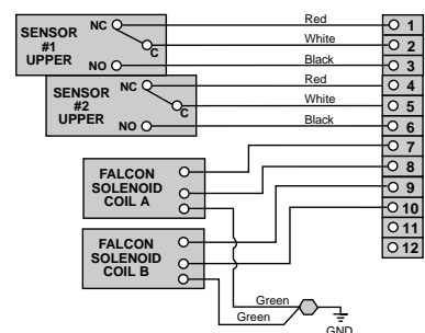
2-SPDT Magnum Sensors with Falcon Dual Coil Solenoid & 12 PT TS
