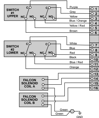
P+F Kriterion Sensor with Falcon Solenoid & 8 PT TS
