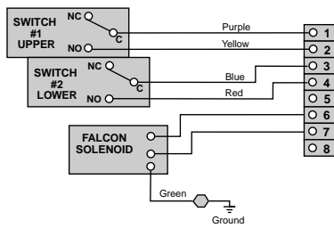
2-SPST Mechanical Switches with Falcon Solenoid & 8 PT TS
