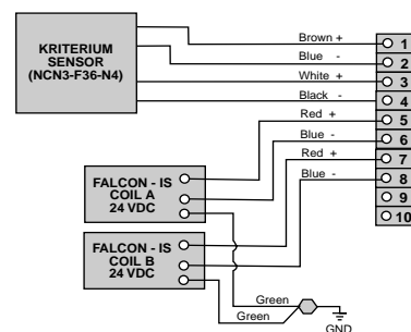
P+F Kriterion Sensor with Falcon Dual Coil Solenoid & 10 PT TS
