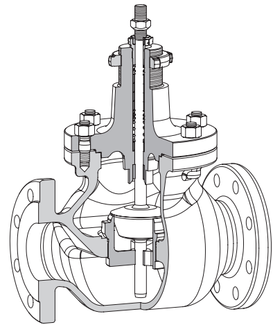
Fig. 1 · Type 3251 Valve with AC-1 Trim
