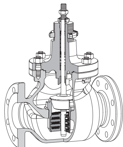
Fig. 2 · Type 3251 Valve and AC-2 Trim with four attenuation plates
